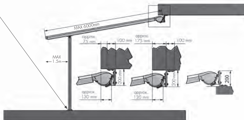
Ceiling installation of VARIO PERGOLA with angle towards the back or towards the front
